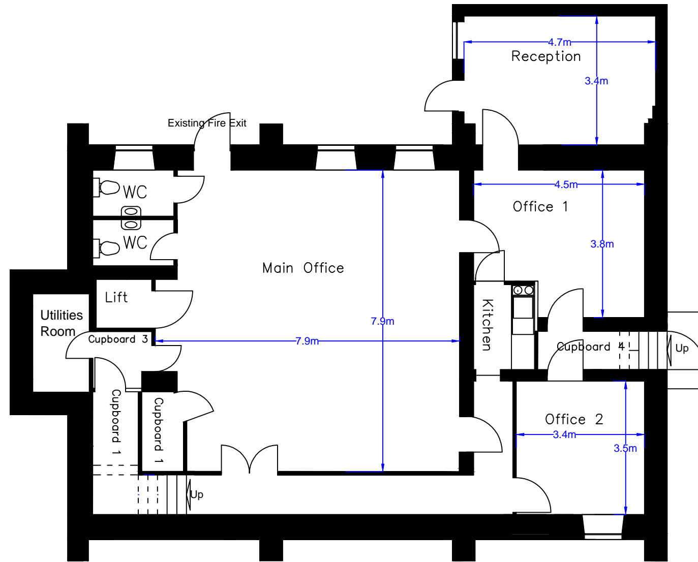
8DT11: 8 Derby Terrace Lower Ground Floor Plan as Is Page 1 of 1, Scale 1:100 at A3
